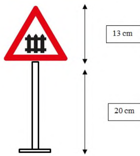
Figure 7. Level crossing signage dimensions
